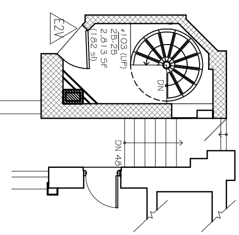
2ND FLOOR
