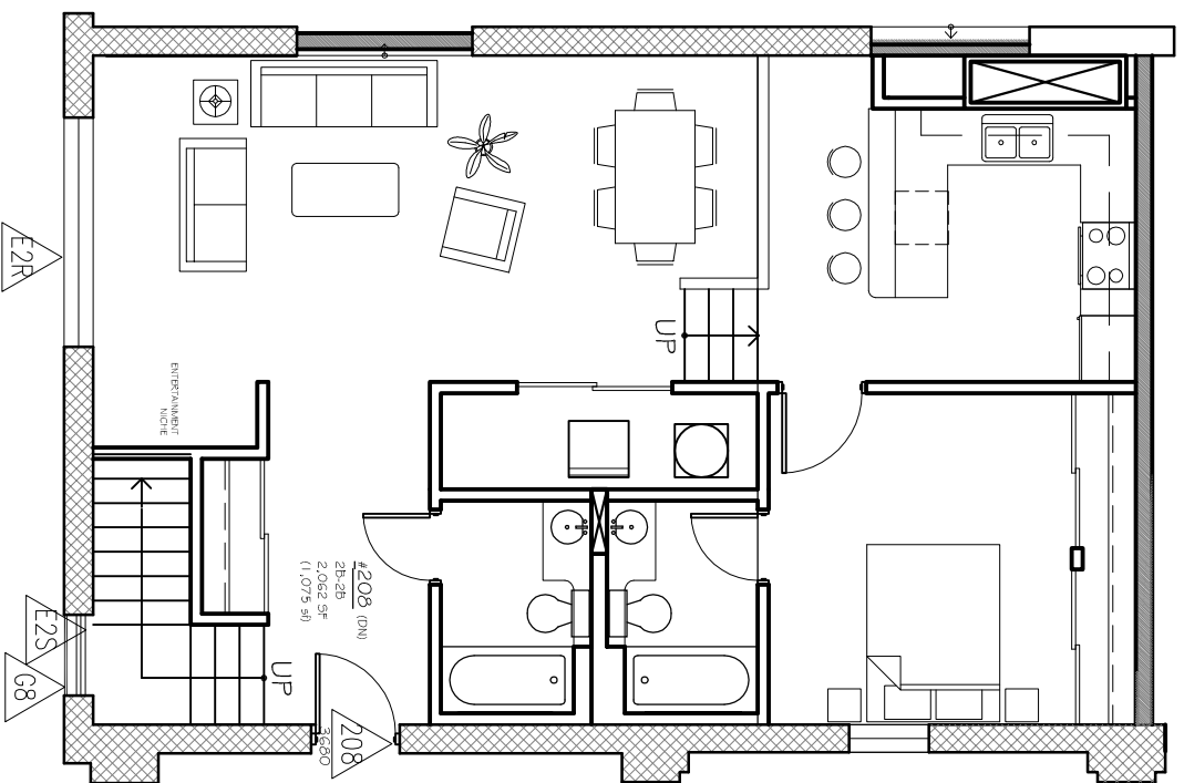
2ND FLOOR
