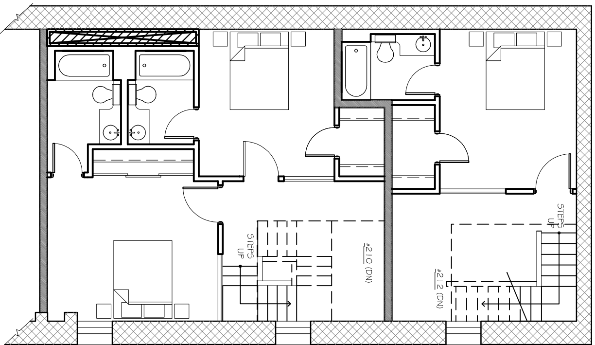
1ST FLOOR
