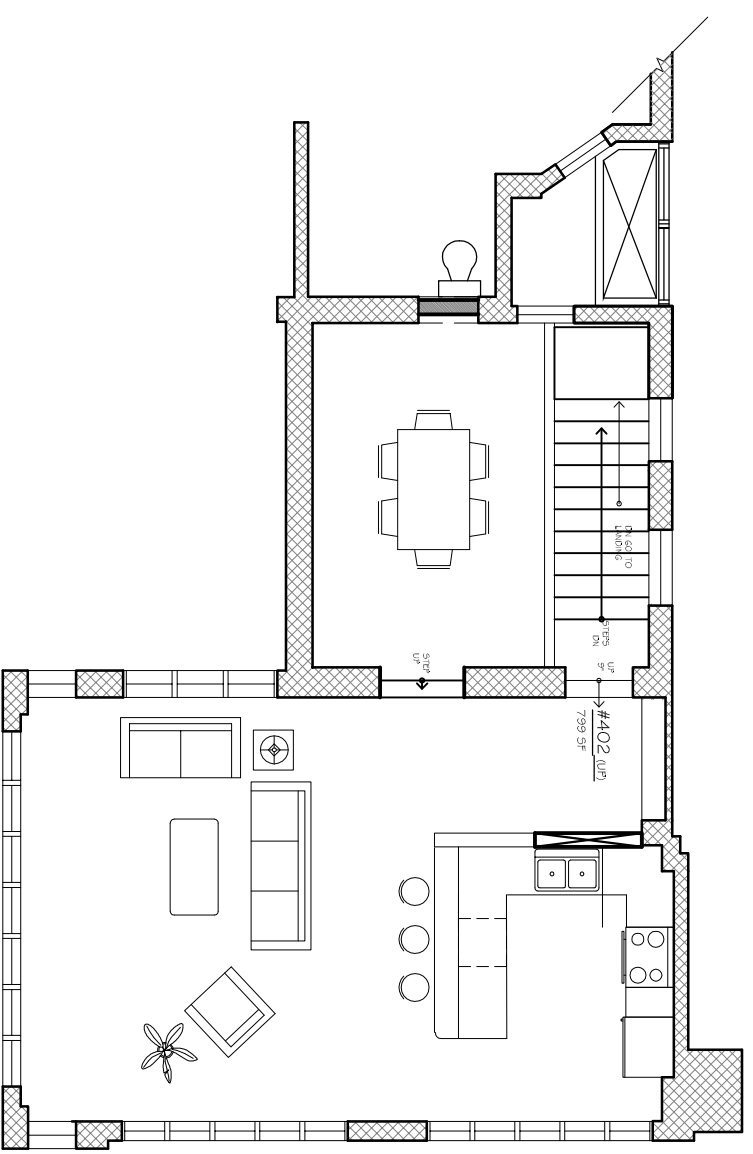
5TH FLOOR
