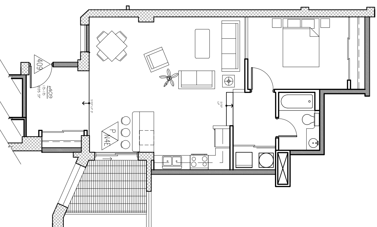
UNIT 409 - 4TH FLOOR
