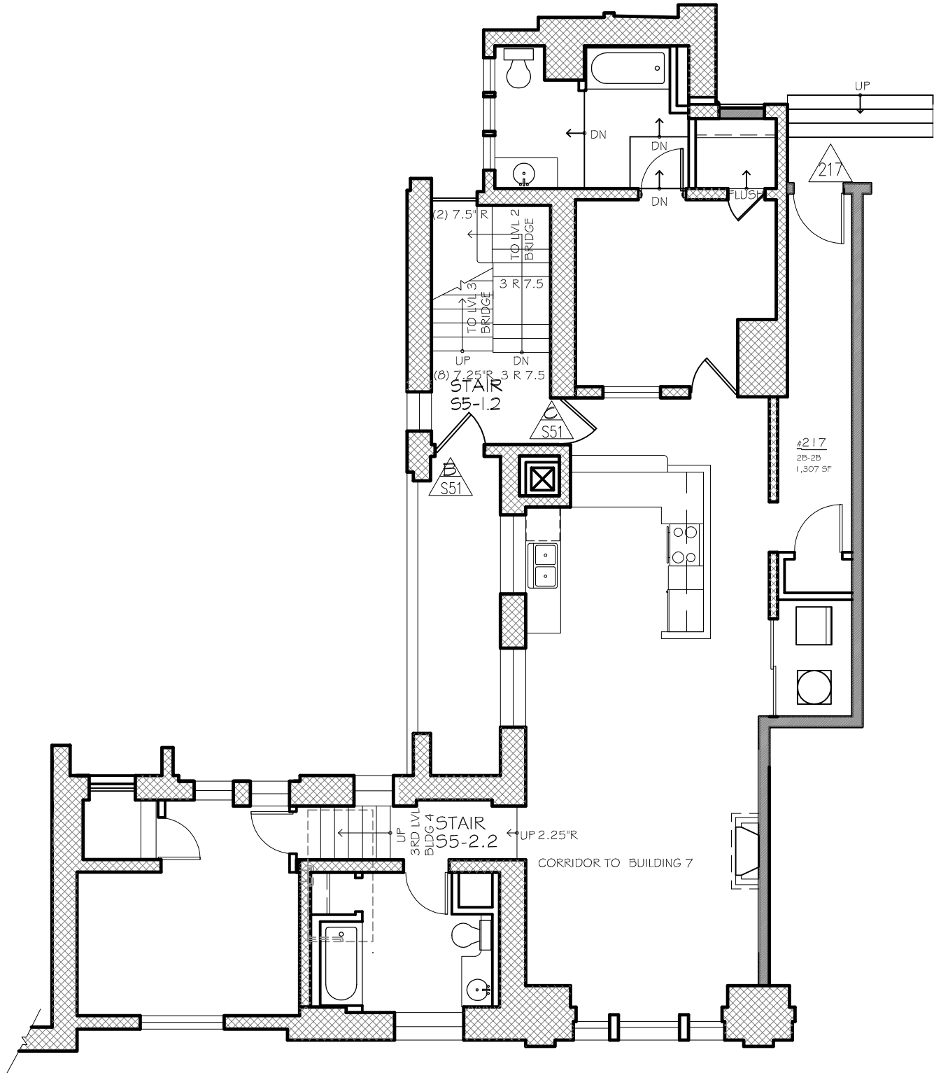
UNIT 217 - FLAT
