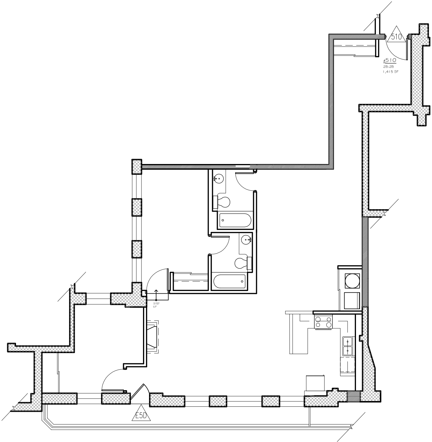
UNIT 510 - 5TH FLOOR
